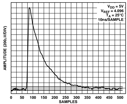
Figure 21. Glitch Energy
